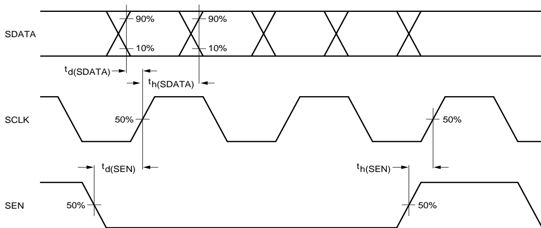
Fig.18 Interface timing for front-end ICs.
